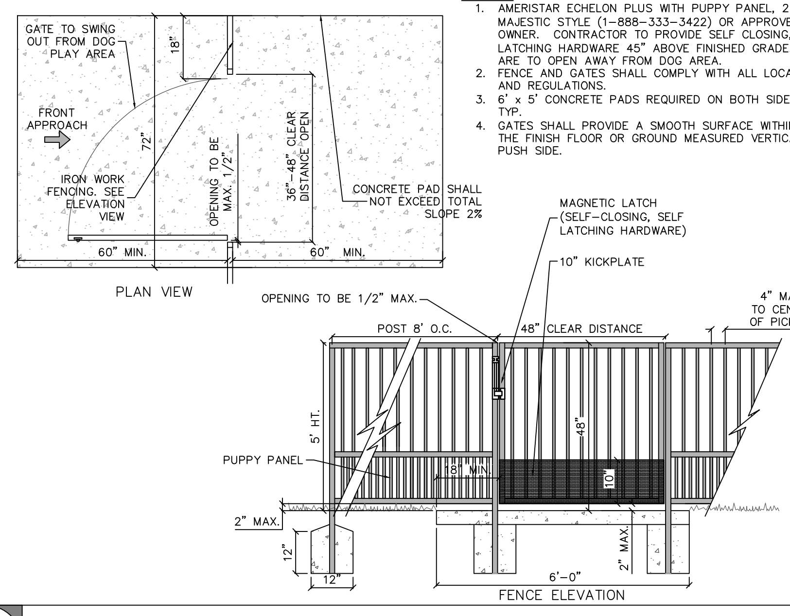
DOG PARK FENCE & GATE DETAIL
